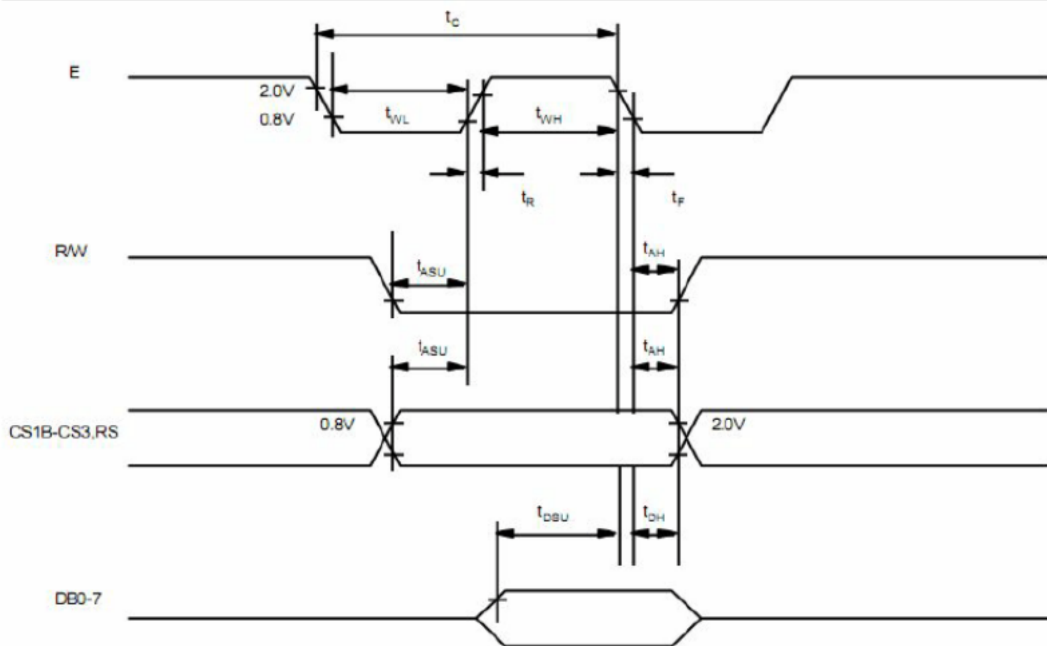
Fig 3. MPU write timing
